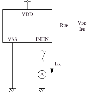
Measurement cct 5
